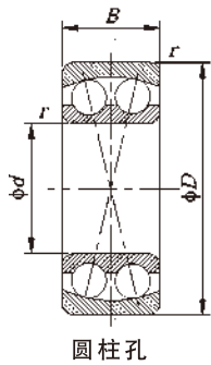
圆柱孔
