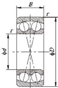
圆柱孔
